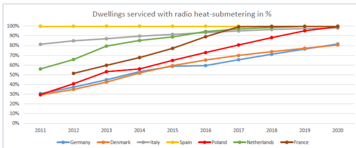
Figure 13: Share of sub-metered dwellings serviced with remote readings (not requiring access to flats) in selected European countries.
