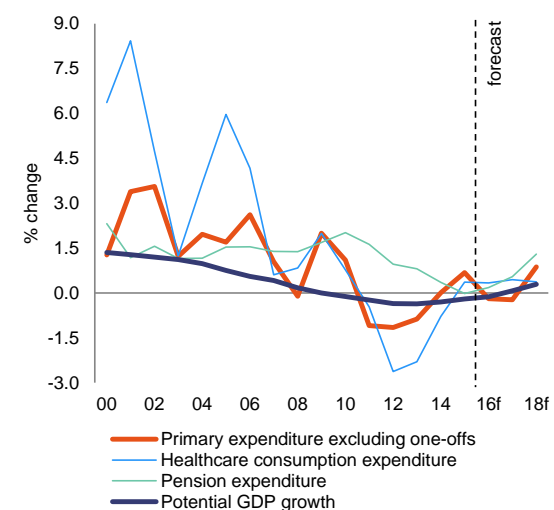
Graph 4.1.1: Evolution of government real primary expenditure and potential GDP growth
