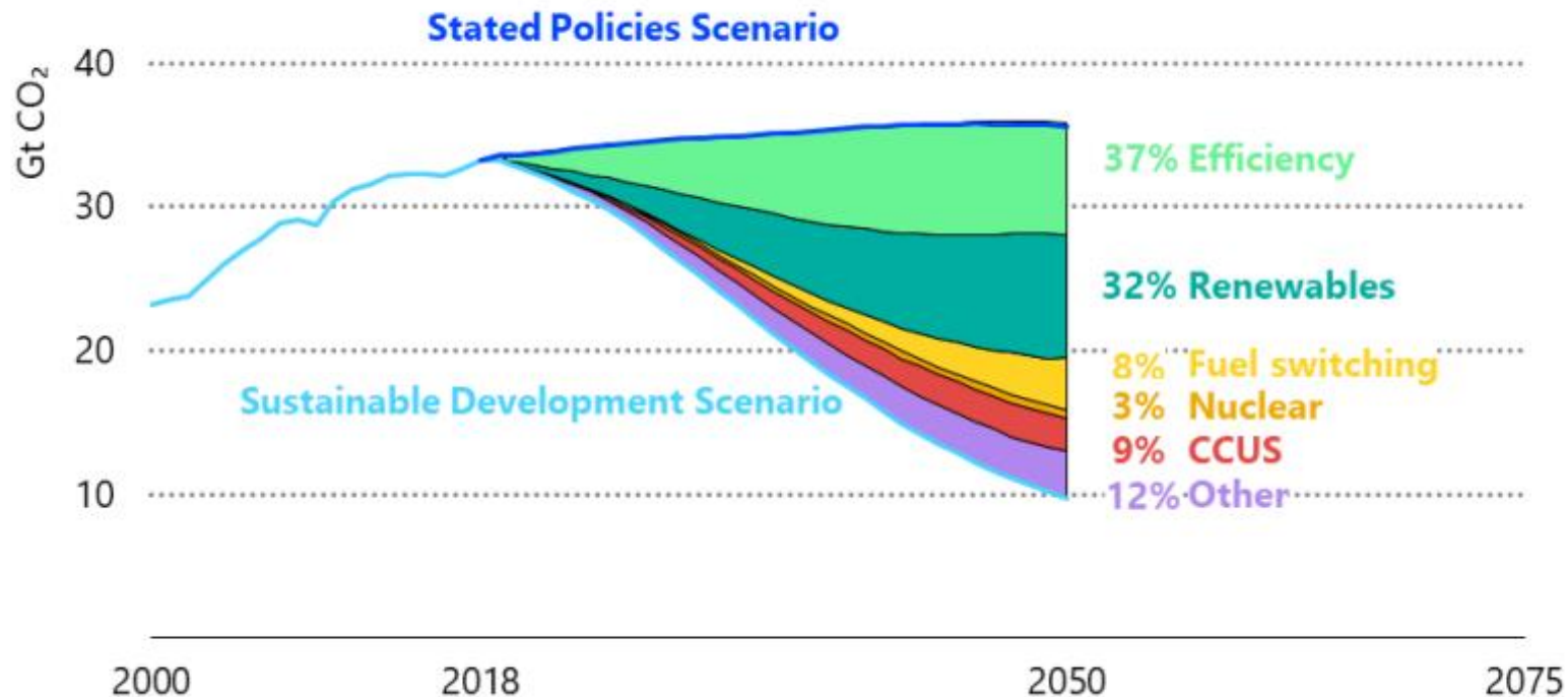
Energy-Related CO 2 Emissions and CO 2 Emissions Reductions by Measure in IEA's Sustainable Development Scenario
