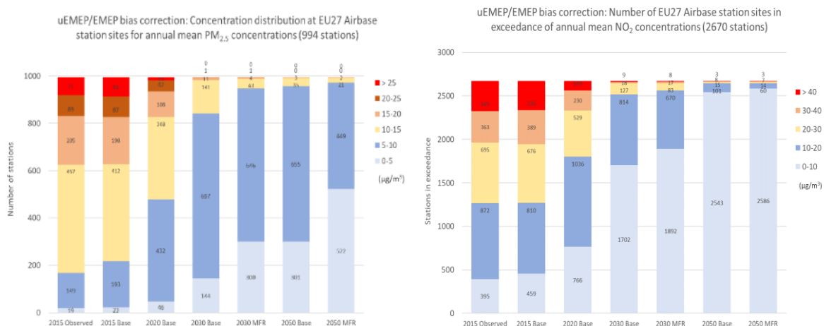
Figure 5 – PM 2.5 (left) and NO 2 (right) concentration modelling outputs for EU under baseline assumption. 48
