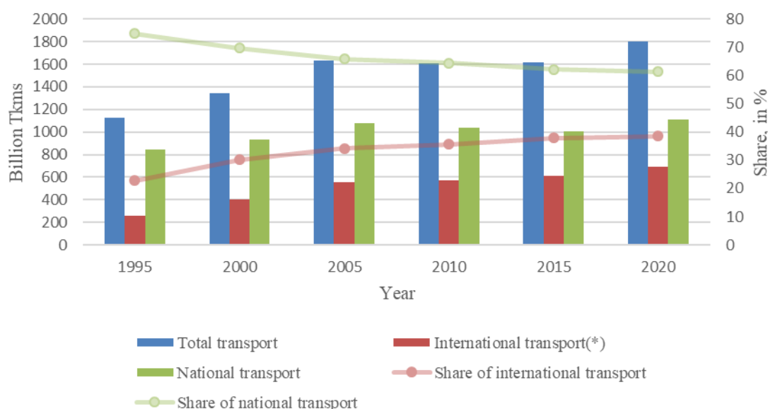
Figure 1: Road freight transport by HDV in the EU, 1995-2020.
