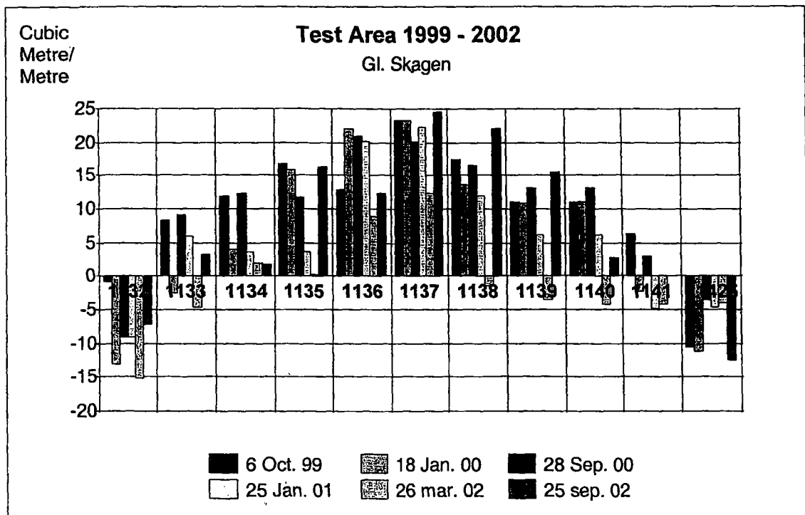
Fig. 4 Test Area Sediment Accumulation
