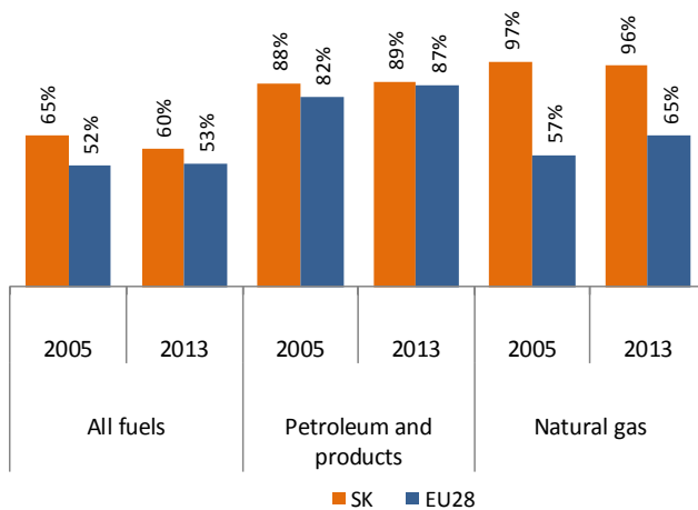
Import dependency 2013
