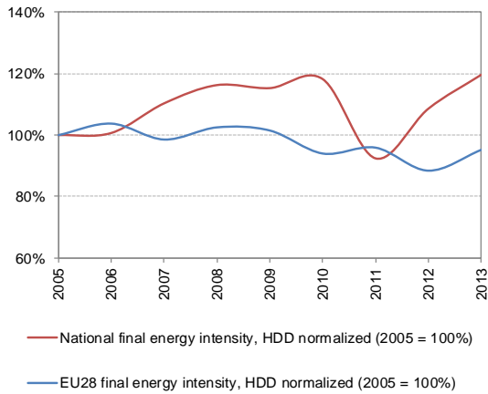
EL) Services: final energy intensity (FEC / value added), HDD normalized
