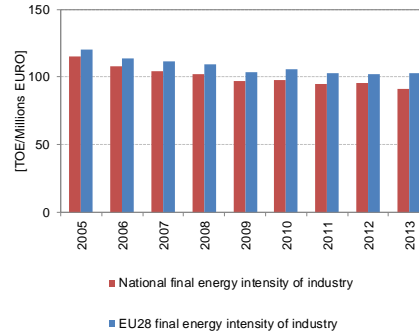
IT) Industry: final energy intensity (FEC / value added)
