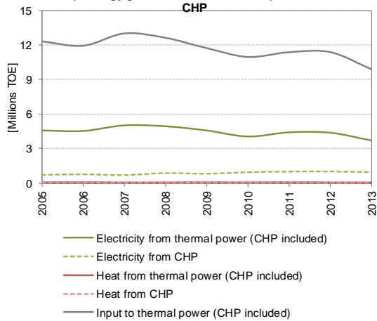
EL) Energy generation from thermal power and CHP
