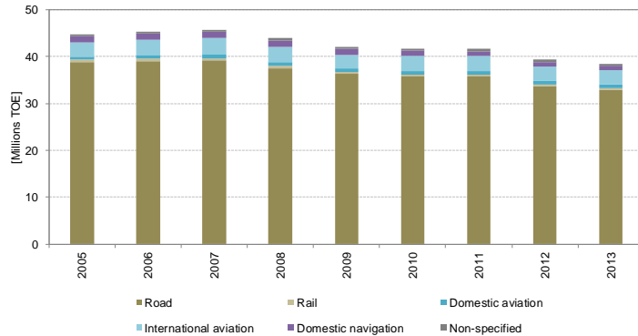
IT) Transport: final energy breakdown
