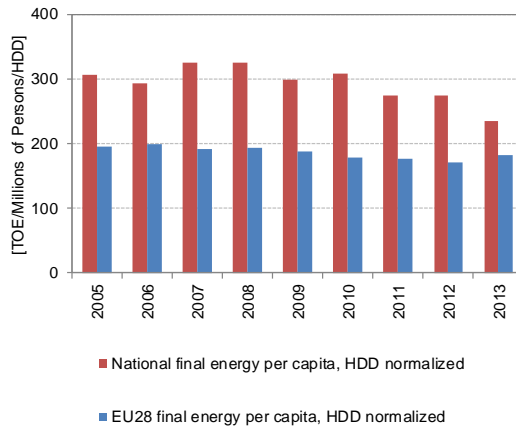
EL) Residential: final energy consumption per capita, HDD normalized
