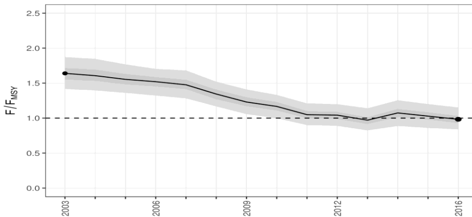
Figure 3 F/F_{MSY} trend
