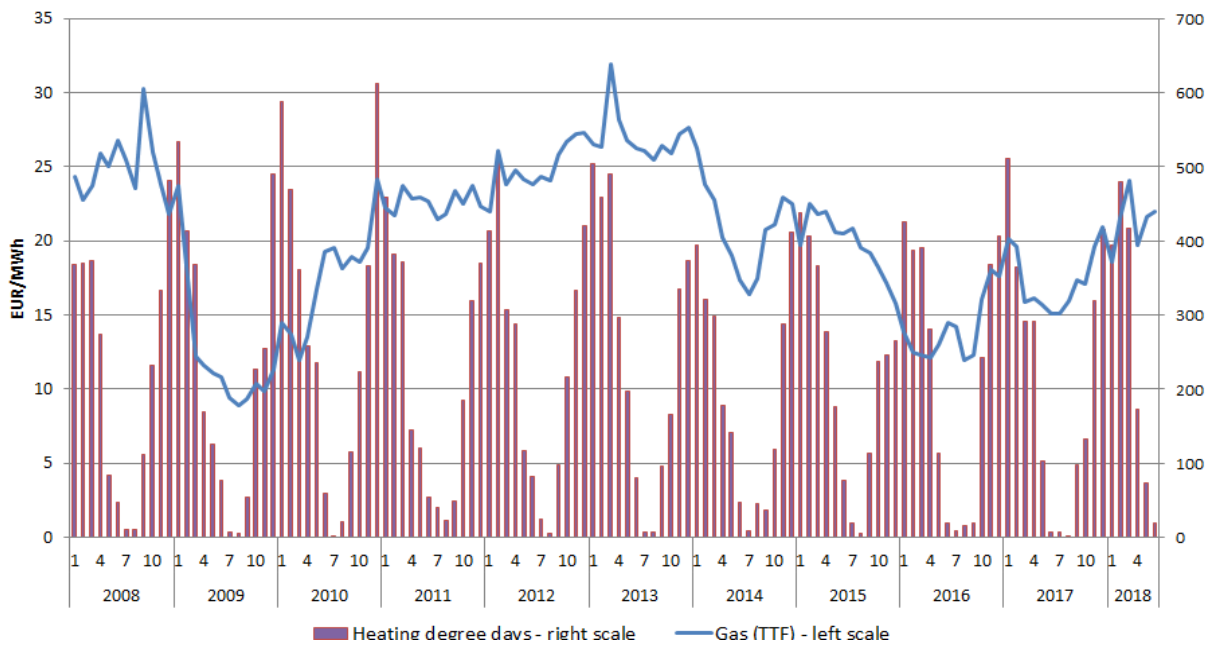
Figure 44 - Monthly average gas price at the Dutch TTF hub and heating degree days in the Netherlands
