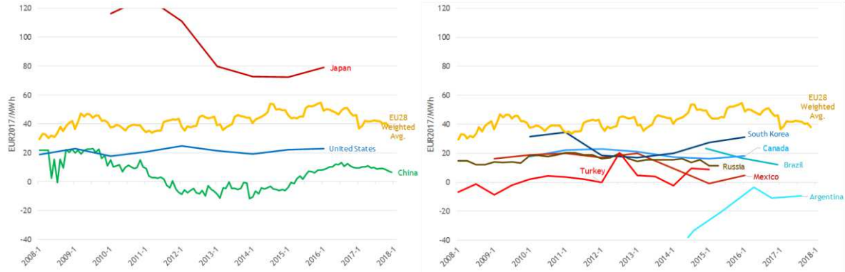
Figure 59 - Difference between household retail natural gas prices and wholesale prices, EU28 and trading partners
