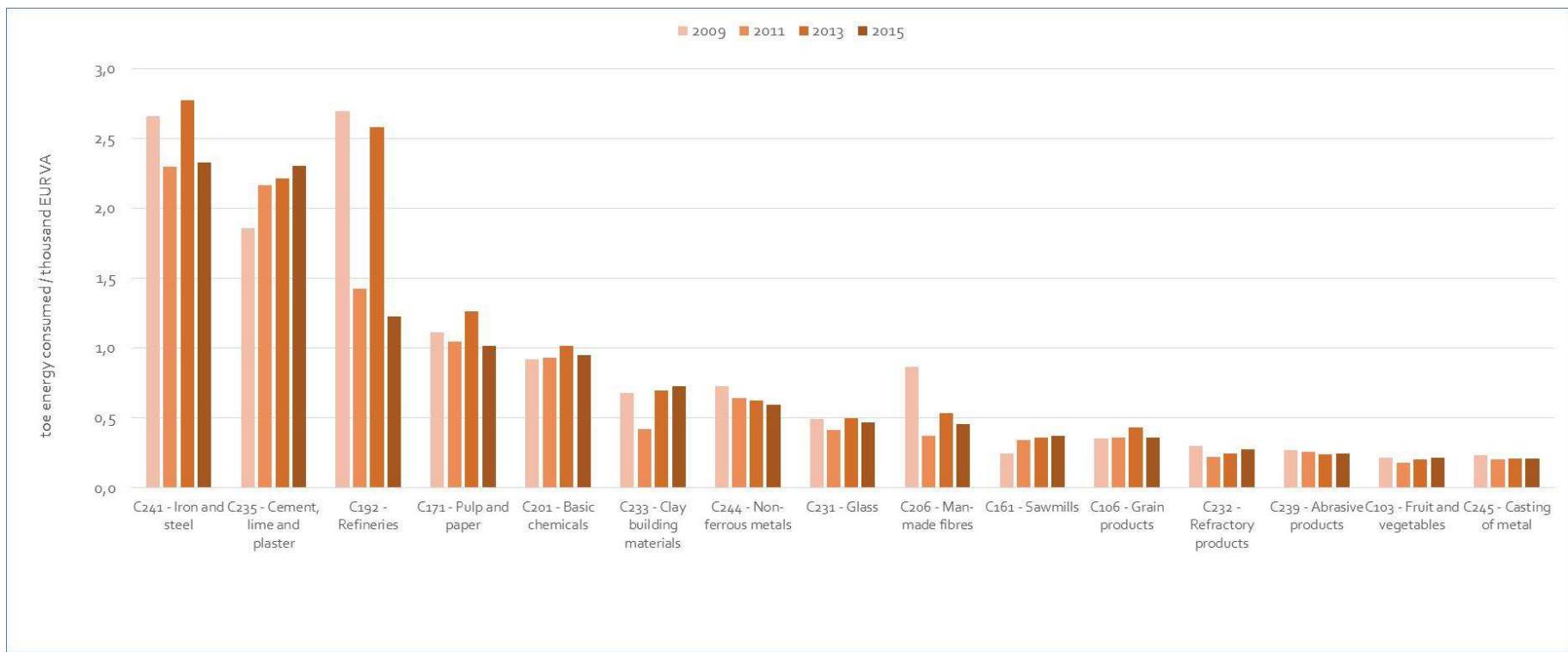
Figure 124 - Energy intensity (consumption/value added in nominal terms) for the most energy intensive manufacturing sectors (average of available countries) 77
