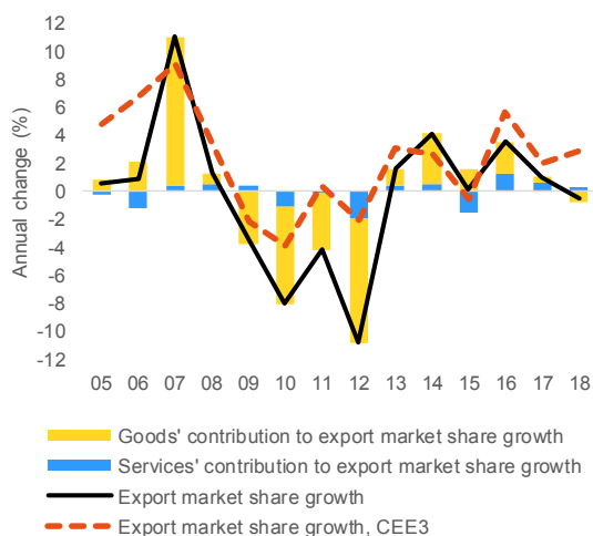
Graph 1.7: Export market share growth
